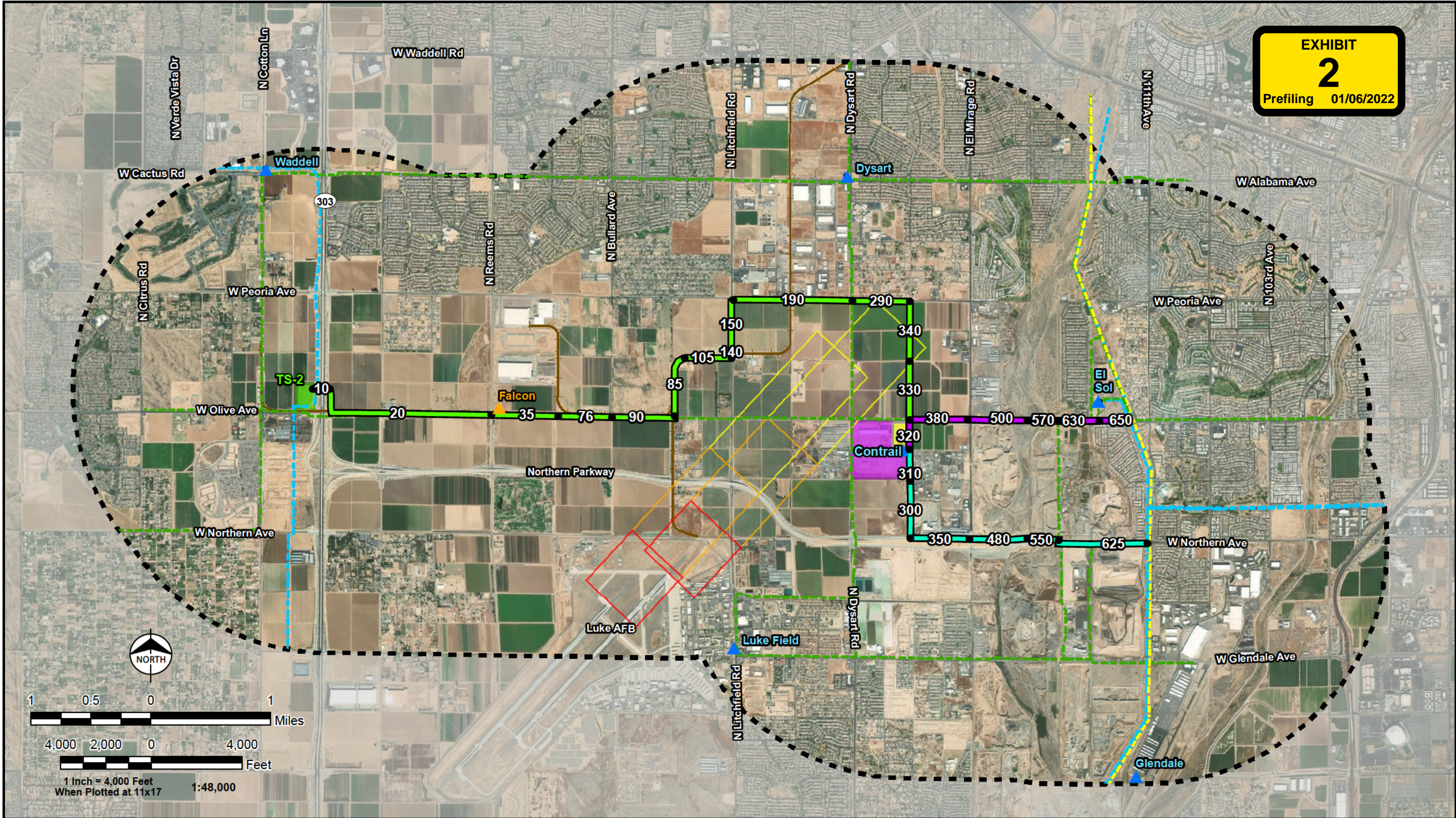
Figure 1 Preferred Routes West Valley Central 230kV Connection Project aps January 2022
