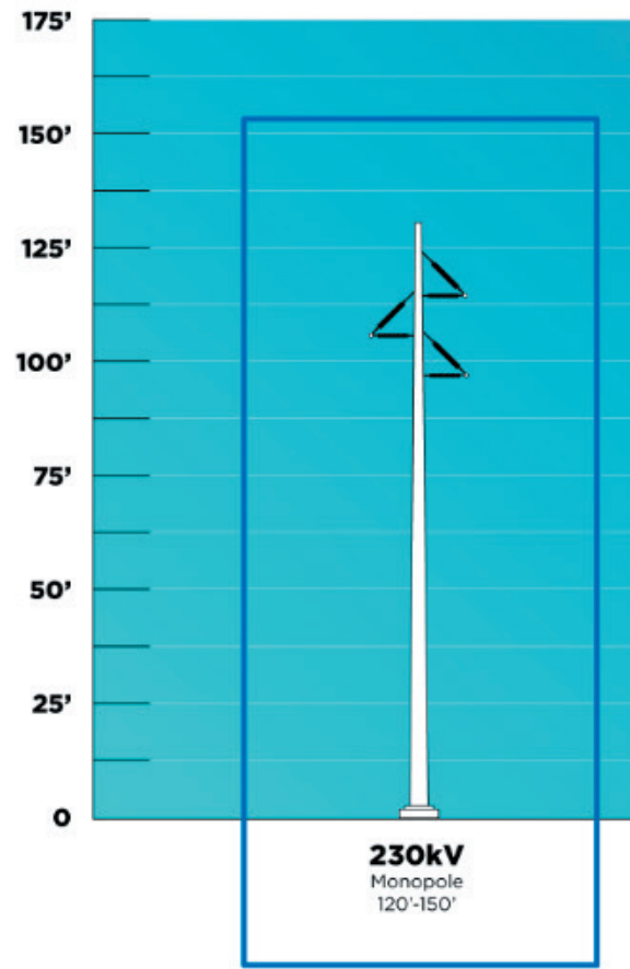
Typical monopole structure
