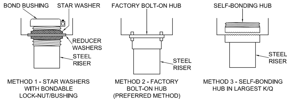
FIGURE 2 - APPROVED METODS FOR METALLIC RISER ATTACHMENT
