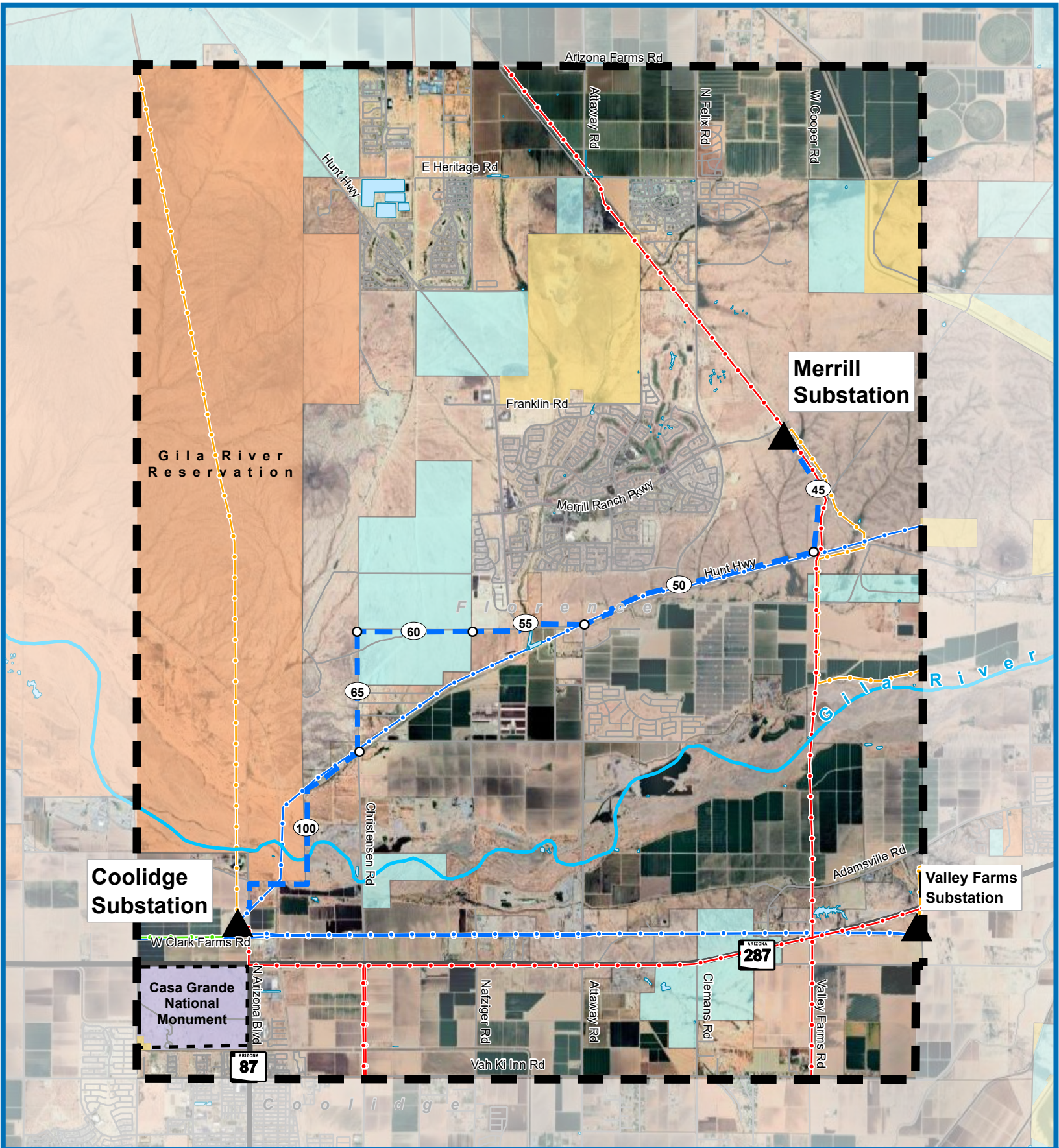
Merrill to Coolidge 69kV Transmission Line Project Figure 6 - Preferred Route
